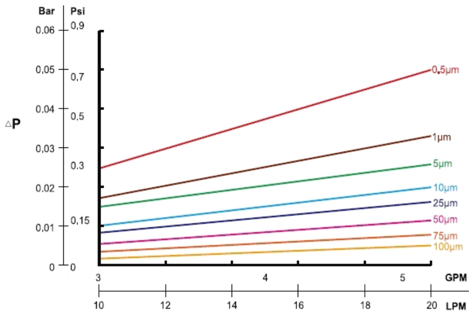
10" PP Filters Flow Rate
