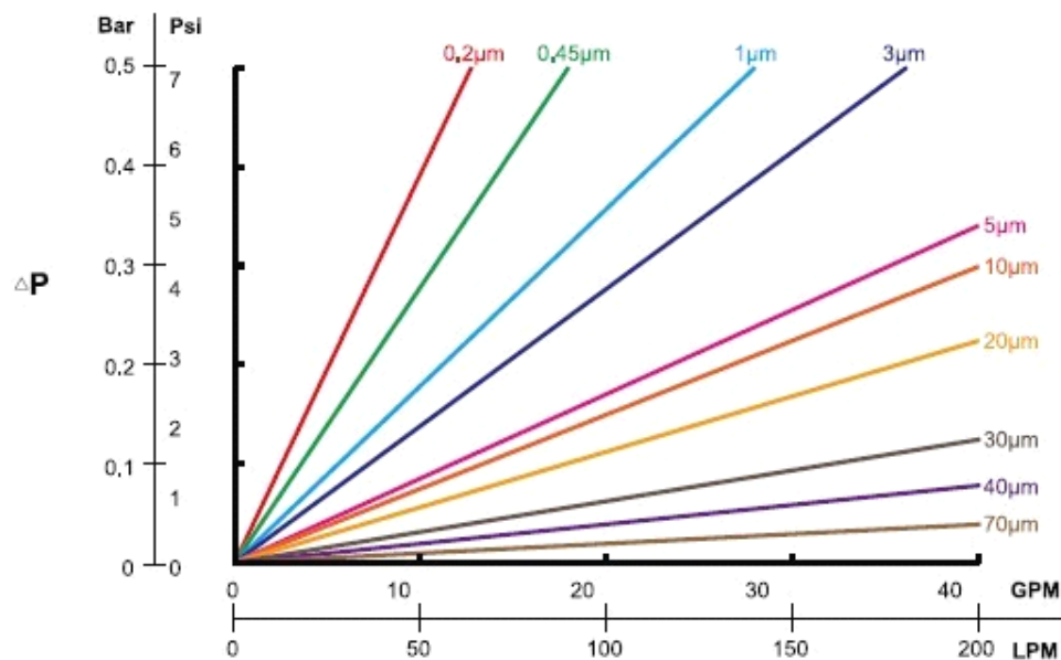
10" Glass Fiber Membrane Pleated Filter Cartridge Flow Rate
