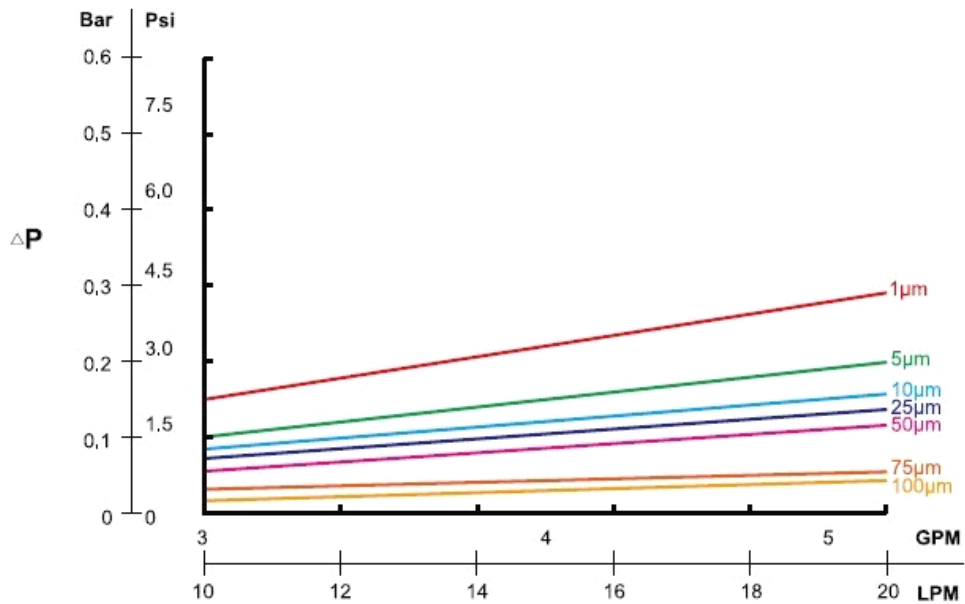
10" PP Filters Flow Rate
