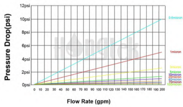
Pressure-Drop Rate for 60" High Flow Cartridges
